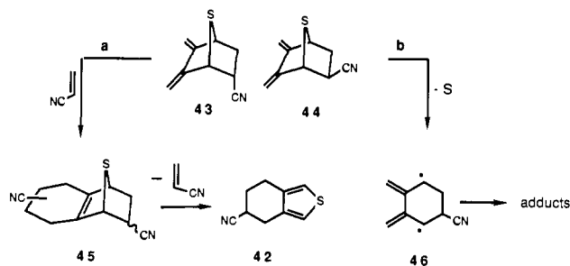
Scheme XII
