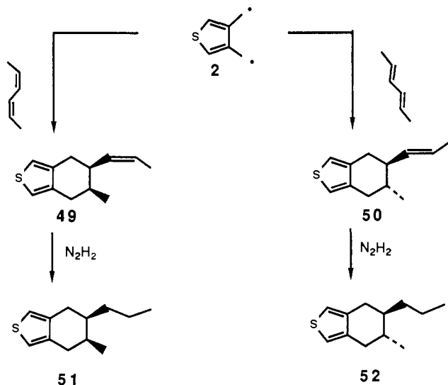
Scheme XIV
